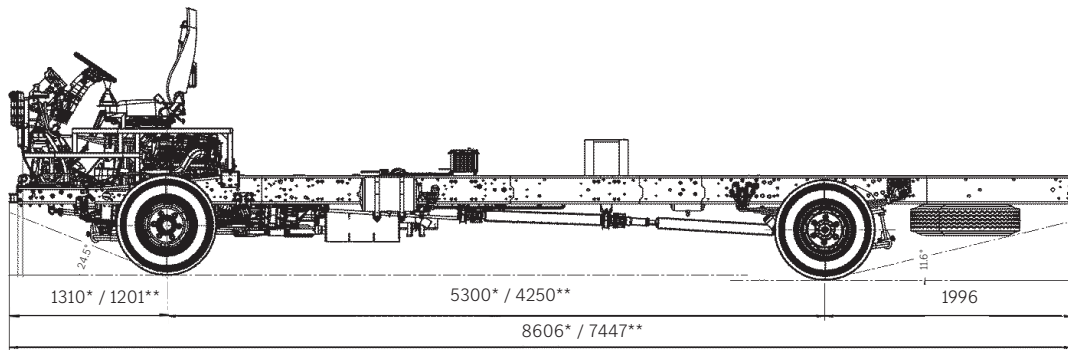
Tampak Samping
